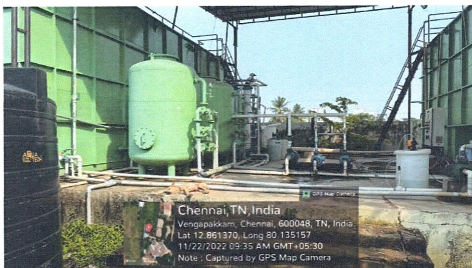
STP Plant
